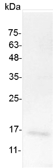
SDS-PAGE analysis of recombinant mouse IL-7
